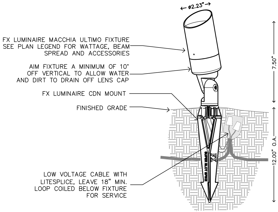
SECTION/ELEVATION
