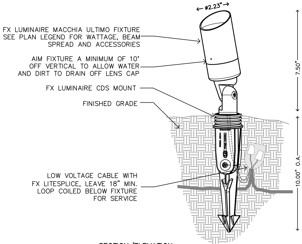
SECTION/ELEVATION
